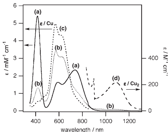
Fig. 6. Electronic spectra of [\text{Cu}(\text{L}^{\text{Me,Bn}})]^+ in acetone; (a) at -90^\circ\text{C} (0.238 mM and P(\text{O}_2) = \sim 1 atm), (b) at -90^\circ\text{C} after bubbling of Ar gas into the former acetone solution for a few minutes, and (c) at -90^\circ\text{C} (1.02 mM and P(\text{O}_2) = \sim 0.02 atm) measured by an optical fiber with a corrected light path length of 0.279 cm, where \epsilon values for [\{\text{Cu}(\text{L}^{\text{Me,Bn}})\}_2(\text{O}_2)]^{2+} should be read as twice as those given in the left hand axis, and (d) at -90^\circ\text{C} (1.01 mM and P(\text{O}_2) = \sim 0.02 atm).
