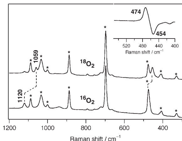
Fig. 10. Resonance Raman spectra of [\text{Cu}(\text{L}^{\text{Me,Bn}})(\text{O}_2)]^+ with 413.1 nm laser excitation in acetone- d_6 at \sim -95 ^{\circ}\text{C} . Inset is a difference spectrum of those of ^{16}\text{O}_2 and ^{18}\text{O}_2 samples. The asterisked bands are solvent bands.
