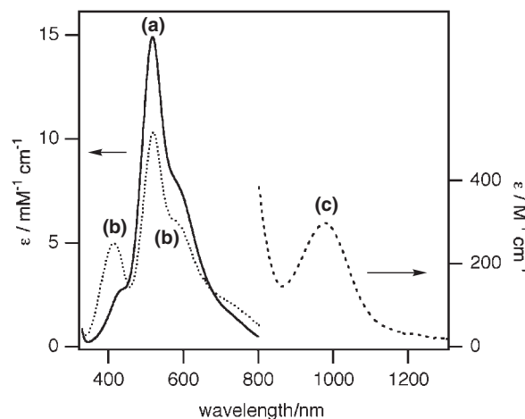
Fig. 5. Electronic spectra of [\text{Cu}(\text{L}^{\text{H,Bn}})]^+ in acetone under P(\text{O}_2) \sim 1 \text{ atm} ; (a) at −80 °C (0.123 mM), (b) at −90 °C (0.117 mM) and (c) at −80 °C (4.04 mM). \epsilon values are given based on a dimer.
